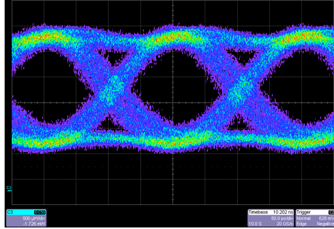
Figure 2: Optical eye diagram of a VCSEL channel coupled to a driver ASIC.
