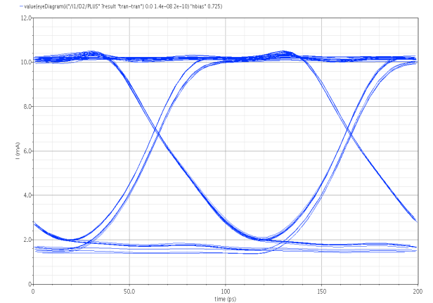
Figure 7: Simulated eye diagram for the VCSEL driver stage operating at 10 Gb/s.
