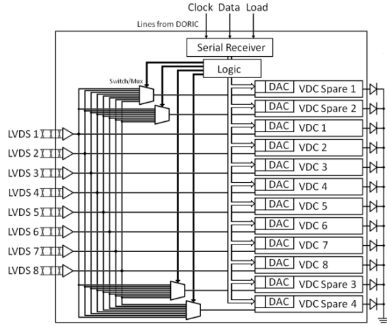
Fig. 1. A 12-channel VCSEL array driver ASIC.
