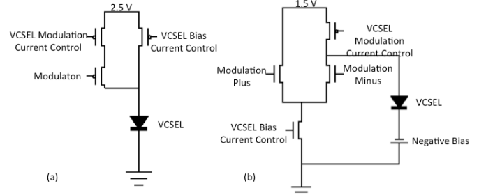
Figure 6: Schematic of a 5 (a) and 10 (b) Gb/s design for the VCSEL driver stage.
