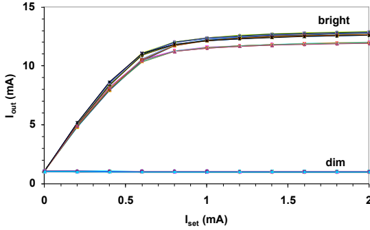
Figure 3: VCSEL drive current vs. I_{\text{set}} of eight 4-channel VDCs.
