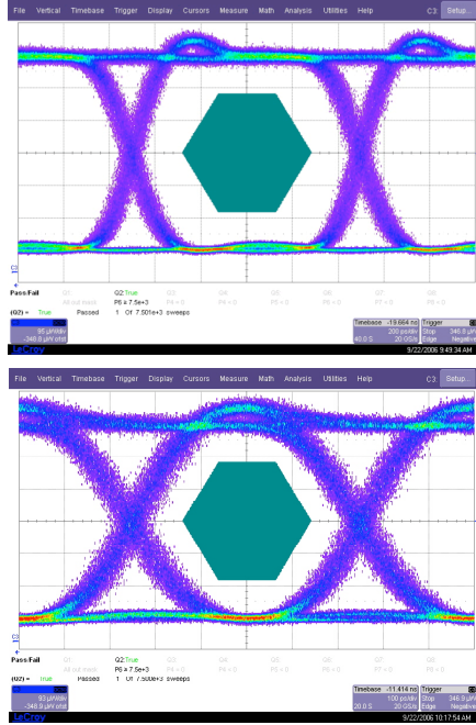
Figure 3: Eye diagrams for optical signals of (a) 1 and (b) 2 Gb/s in a fusion spliced SIMM/GRIN fiber.
