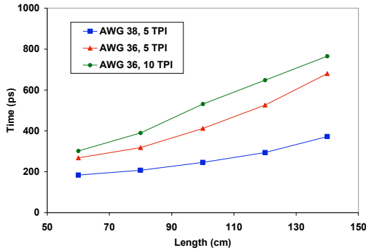
Figure 1: The rise times (20-80%) of the micro twisted-pairs vs. wire length for wires of various diameters and TPI. The fall time distribution has similar characteristics.
