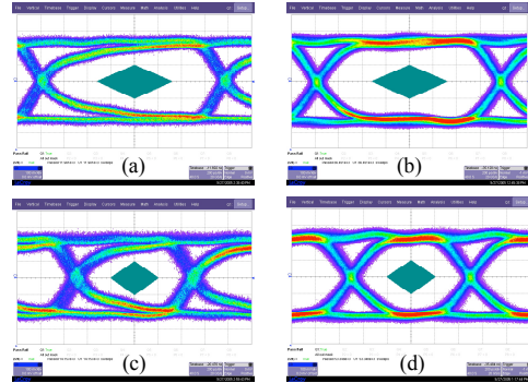
Figure 2: Eye diagrams for signals of (a) 650 Mb/s and (c) 1 Gb/s in a barrel cable of 1.4 m. (b,d) show the corresponding signals for a cable of 0.8 m.
