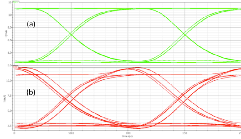
Figure 7: Eye diagrams at 10 Gb/s for the new 10 Gb/s (a) and existing 5 Gb/s (b) designs of the VCSEL driver stage.
