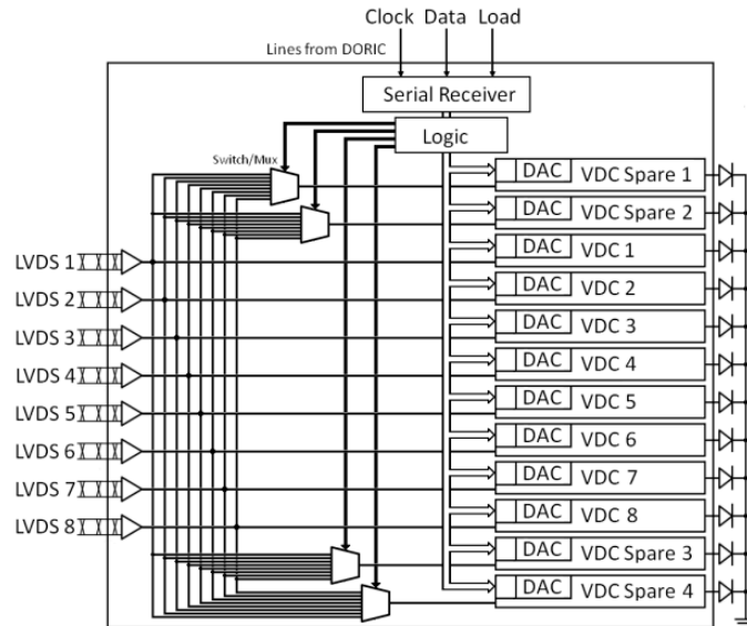
Figure 1: A 12-channel VCSEL array driver ASIC.
