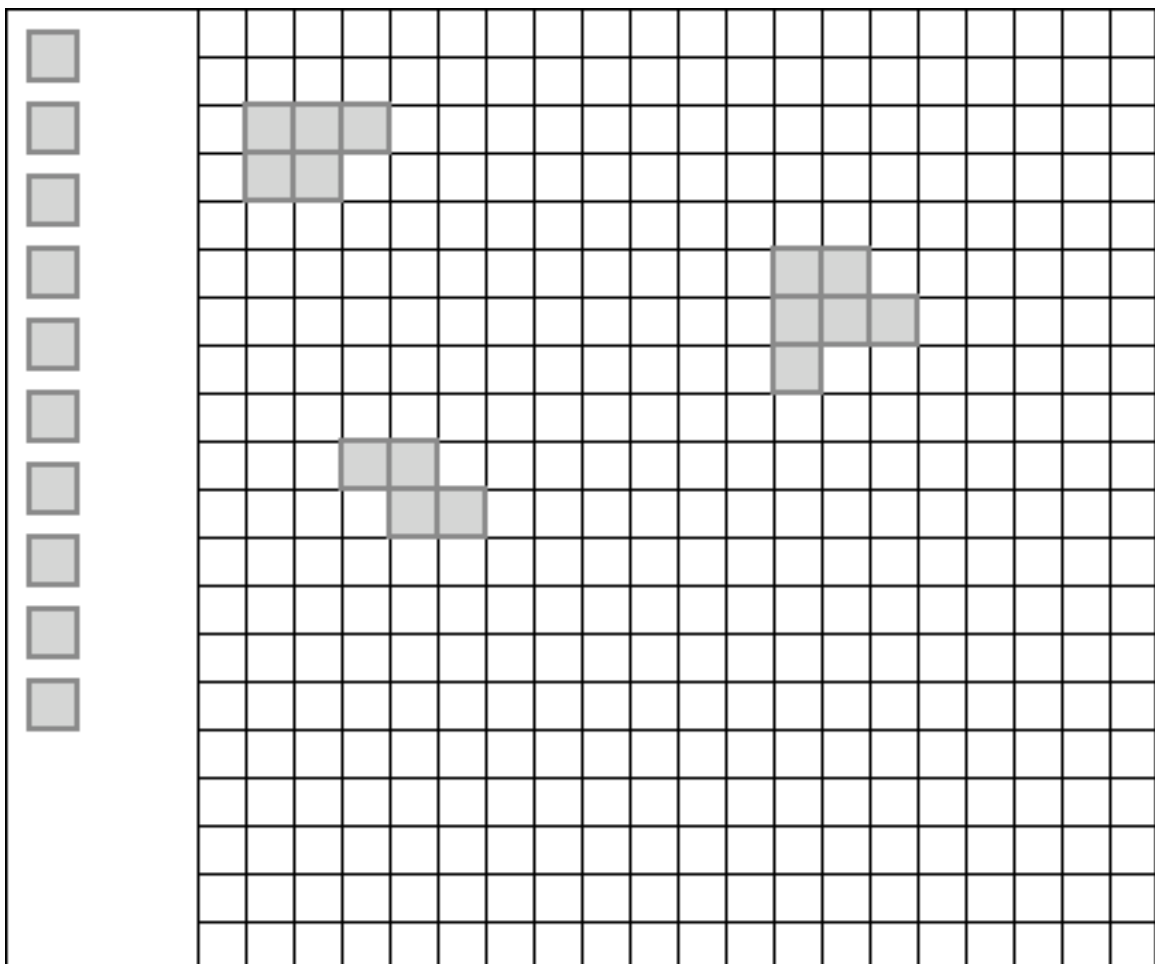
Figure 1. Schematic of the free classification display.
