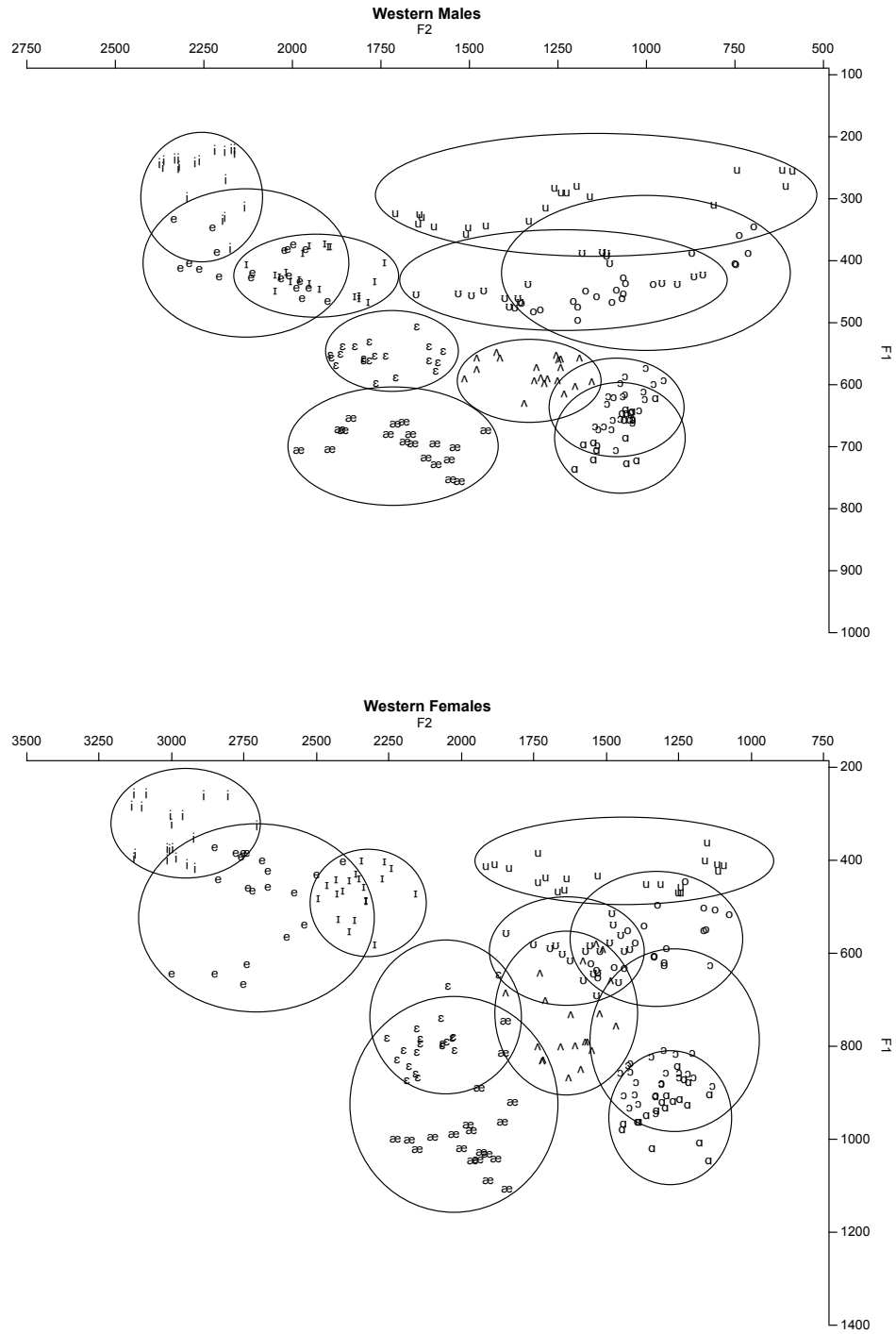
Figure 11. All tokens produced by the Western male (top) and female (bottom) talkers for the 11 vowels [i ɪ e ε æ ɔ ʌ o u]. The ellipses were hand-drawn to include every token for each vowel.
