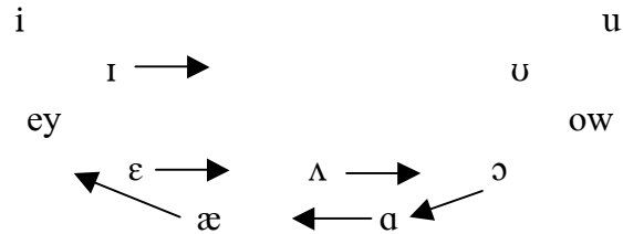
Figure 2. The Northern Cities Chain Shift.
