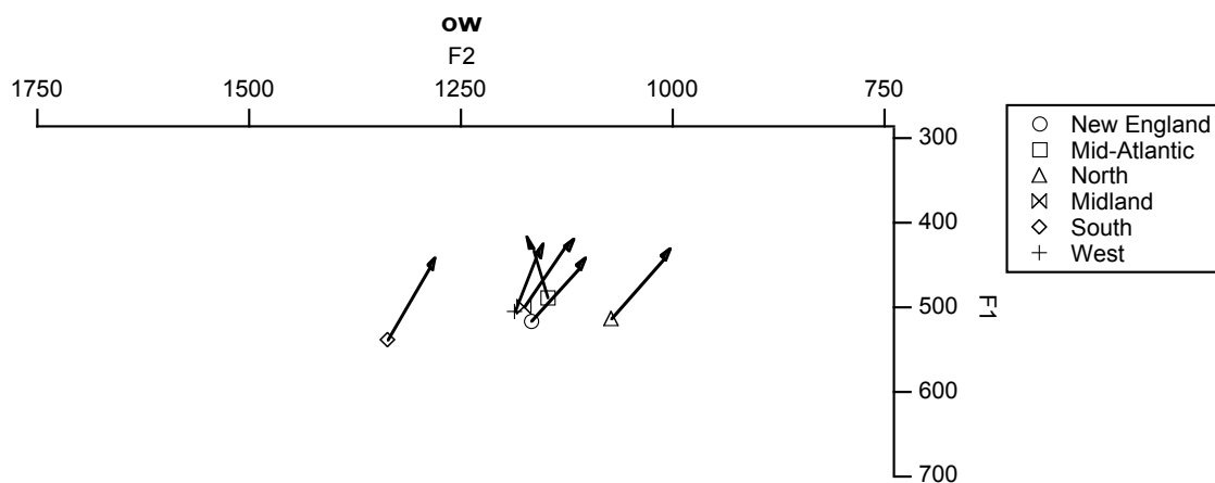
Figure 18. Mean formant frequency trajectories for each dialect for the vowel [o].
