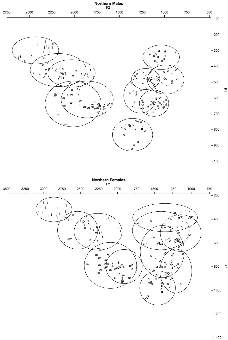
Figure 8. All tokens produced by the Northern male (top) and female (bottom) talkers for the 11 vowels [i I e ε æ a ɔ ʌ o u]. The ellipses were hand-drawn to include every token for each vowel.
