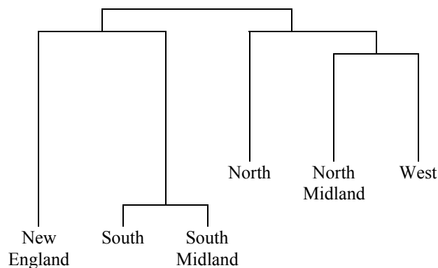
Figure 2. Clustering solution for the listeners in Experiment 1.
