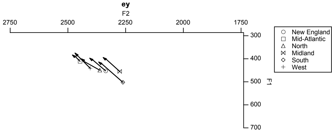
Figure 13. Mean formant frequency trajectories for each dialect for the vowel [e].
