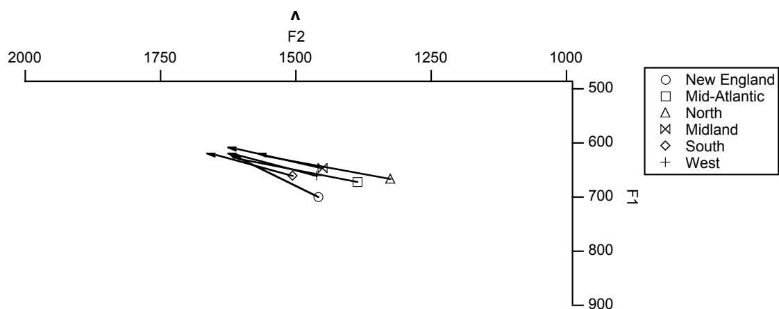
Figure 17. Mean formant frequency trajectories for each dialect for the vowel [ʌ].
