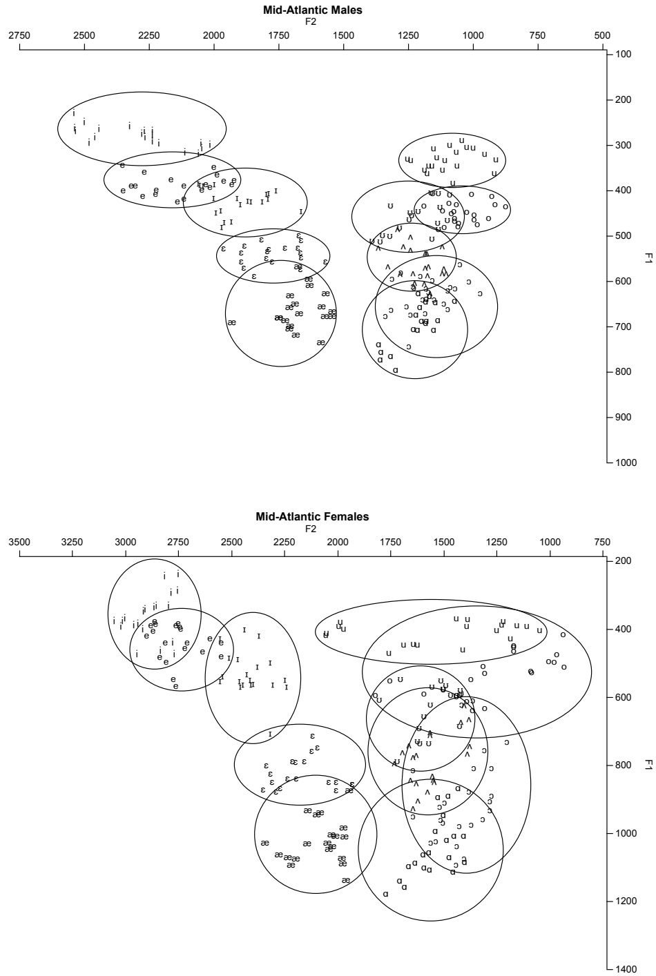
Figure 7. All tokens produced by the Mid-Atlantic male (top) and female (bottom) talkers for the 11 vowels [i ɪ e ε æ ʌ ɔ ʊ u]. The ellipses were hand-drawn to include every token for each vowel.
