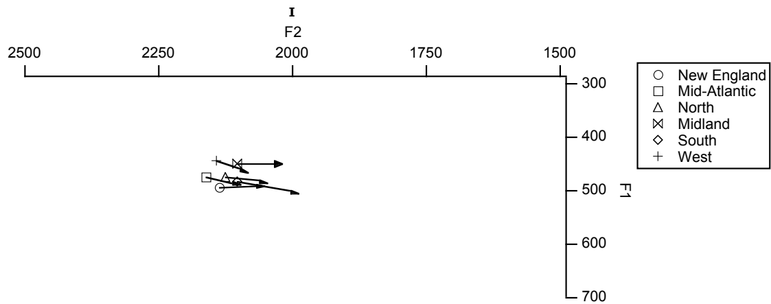
Figure 20. Mean formant frequency trajectories for each dialect for the vowel [ɪ].
