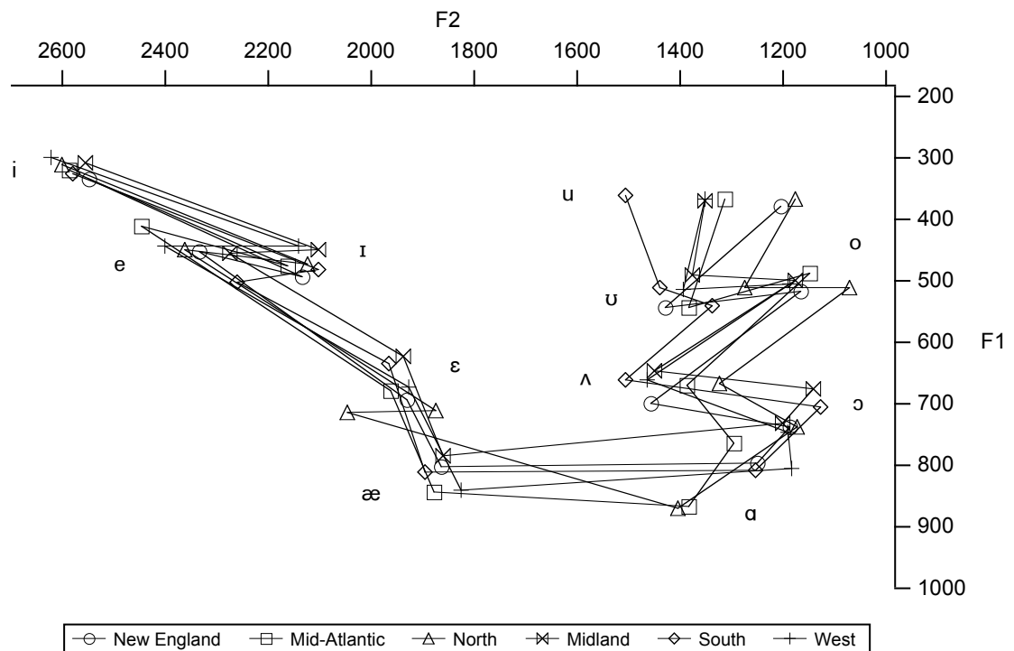
Figure 5. Mean formant frequency values for 11 American English vowels for each of the six dialects. The lines connecting the vowels proceed in a counterclockwise direction as follows: [i I e ε æ α ɔ ʌ o u].
