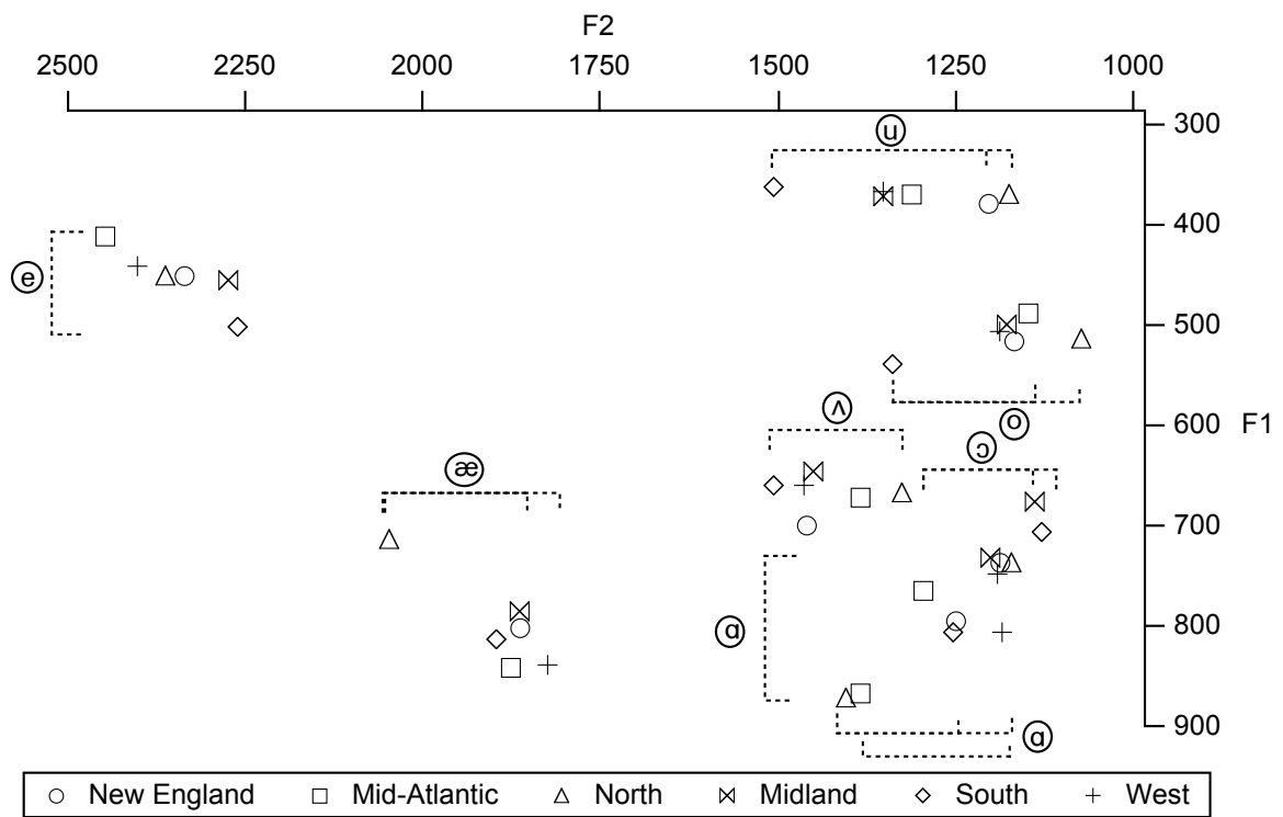
Figure 12. Mean formant frequency values for each dialect for the vowels [e, æ, ɑ, ɔ, ʌ, o, u]. Significant differences based on Tukey tests at the .001 level are depicted by the dashed square brackets.
