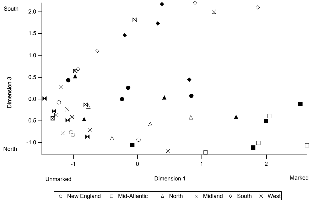
Figure 6. Multidimensional scaling solution for the listeners in Experiment 2 (Dimensions 1 and 3). The filled symbols represent male talkers and the empty symbols represent female talkers. For the West, plain X's indicate females and boxed X's indicate males.
