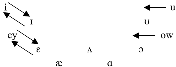
Figure 3. The Southern Vowel Shift.
