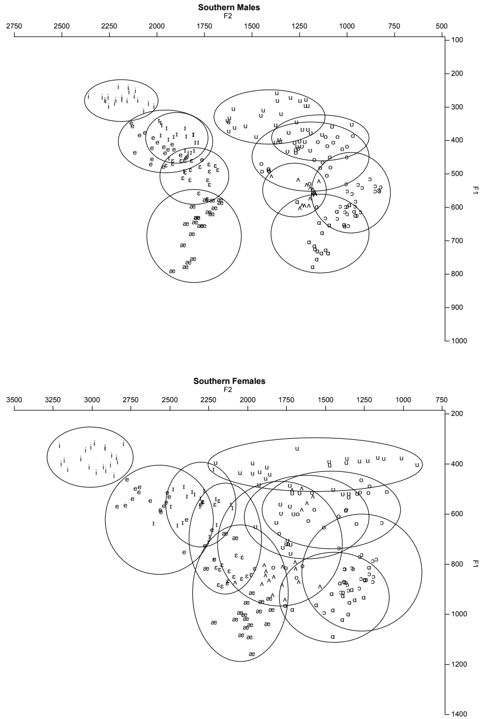
Figure 10. All tokens produced by the Southern male (top) and female (bottom) talkers for the 11 vowels [i I e ε æ a ɔ ʌ o u]. The ellipses were hand-drawn to include every token for each vowel.
