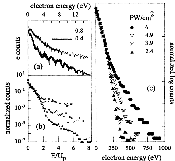
FIG. 2. Helium photoelectron spectra for 780 nm excitation. Low energy electrons plotted in (a) for 0.4 and 0.8 PW/cm ^2 . Scaled energy, E/U_p , plot at (b) 0.2 (crosses), 0.4 (circles), and 1.0 (triangles) PW/cm ^2 . The value of U_p is defined by the laser's peak intensity. Plot (c) shows the high energy electron tail (solid circles) resulting from the sequential formation of He^{2+} .
