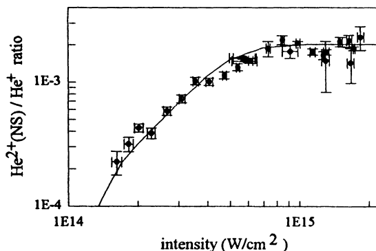
FIG. 3. Intensity dependence of \text{He}^{2+}(\text{NS})/\text{He}^+ ratio. Error bars indicate 1 standard deviation. Solid line is calculated; see text for details. The measured intensities are multiplied by 1.15.
