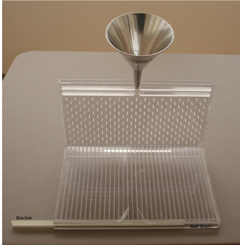
Fig. 1: A picture of the apparatus for demonstrating the C.L.T.
