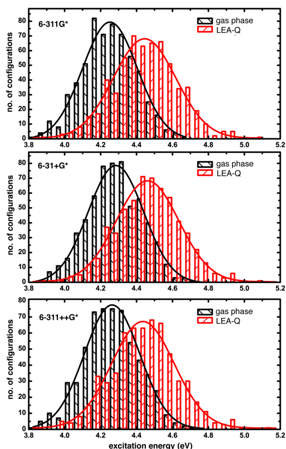
Figure 4. Calculated n \rightarrow \pi^* excitation energies for aqueous acetone by the TD-PBE0 level using various basis sets. The curves are Gaussian fits to the statistical distributions of excitation energies.
