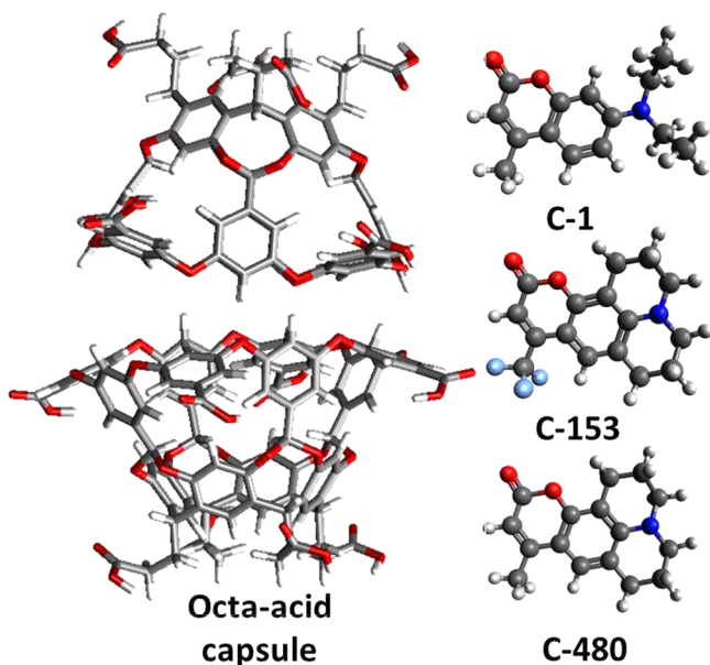
Figure 1. Octa-acid capsule and the guest coumarins: C-1 ( C_{14}H_{17}NO_2 ), C-153 ( C_{16}H_{14}F_3NO_2 ), and C-480 ( C_{16}H_{17}NO_2 ). The atomic coordinates are provided in the Supporting Information.
