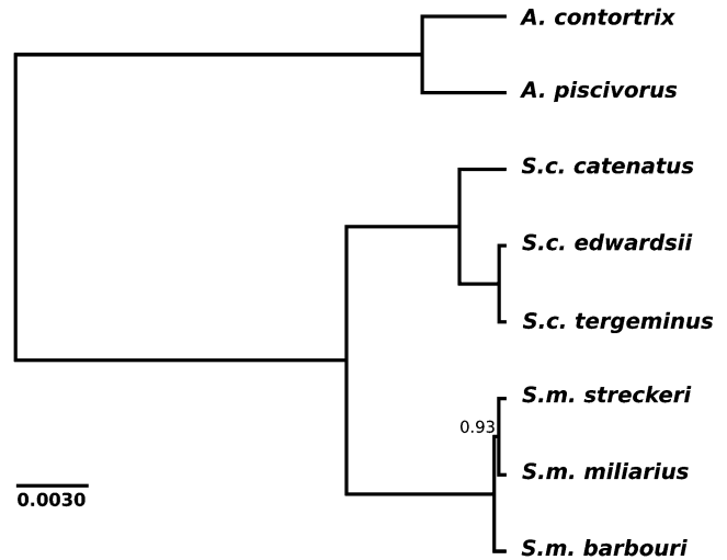
FIGURE 3. Most probable species tree from *BEAST. Branch lengths are scaled according to expected number of substitutions at the TBP locus. The 0.93 represents the posterior probability of the S. m. miliarius and S. m. streckeri clade. All other clades have posterior probabilities in excess of 0.99.
