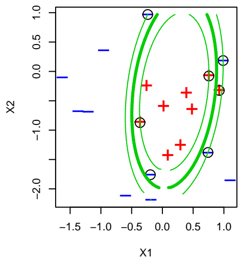
lambda= 0.00836
