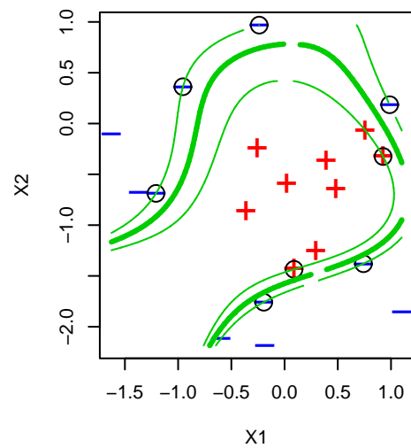
lambda= 0.53
