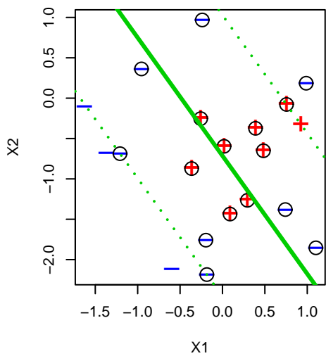
lambda= 1.28
