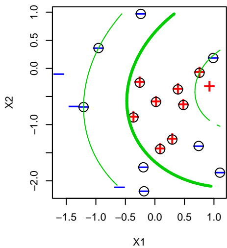
lambda= 0.00665
