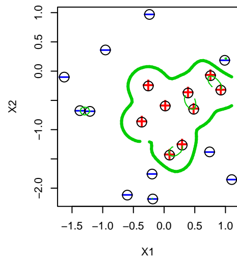
lambda= 0.897
