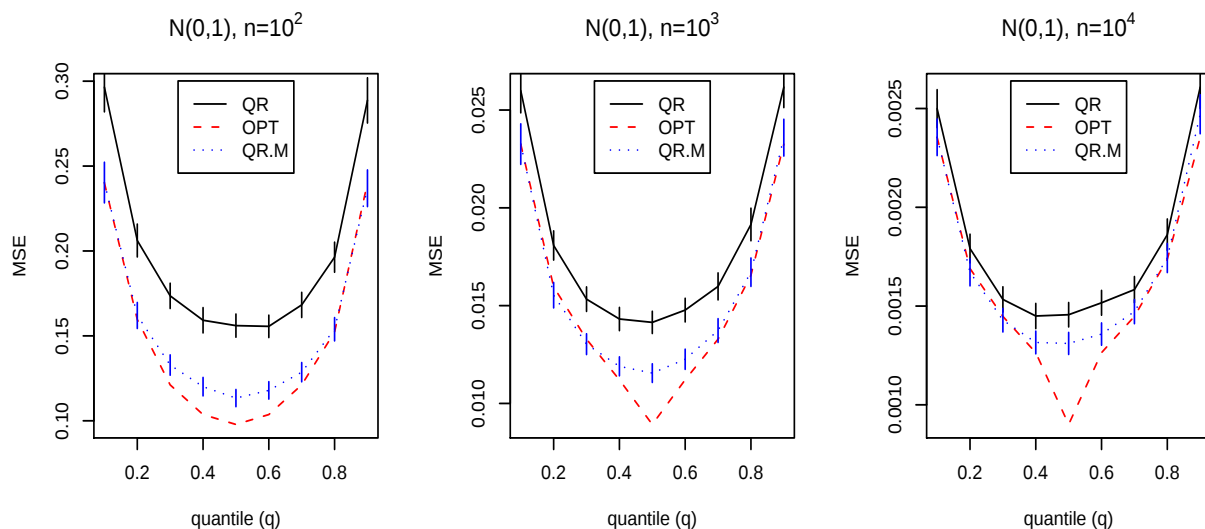
Figure 6: \widehat{MSE} values from quantile regression (QR), modified quantile regression with optimal window width (OPT), and modified quantile regression using the rule (QR.M) under a standard normal error distribution.
