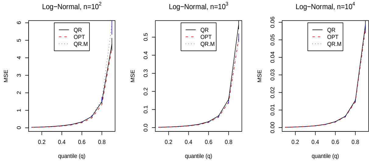
Figure 10: \widehat{MSE} values from quantile regression (QR), modified quantile regression with optimal window width (OPT), and modified quantile regression using the rule (QR.M) under a log-normal error distribution.
