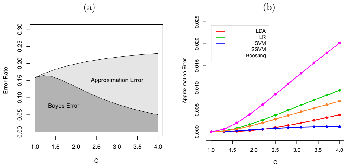
Figure 3: (a) Decomposition of the minimum linear classification error into the Bayes error and the approximation error; (b) Method-specific approximation error of linear classifiers in the QDA setting with \Delta = 2 , \Sigma = I , p = 10 , and \pi_+ = \pi_- .
