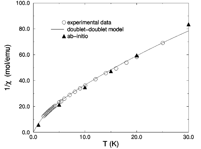
FIG. 8. Inverse susceptibility of (\text{Tb}_{0.02}\text{Y}_{0.98})_2\text{Ti}_2\text{O}_7 . Circles indicate measured values while the solid line is a fit using Eq. (3.3) using a doublet-doublet gap of \Delta = 18 K. The solid triangles are the values obtained from the theoretical calculations of Appendix B.
