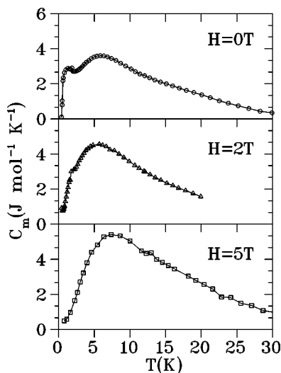
FIG. 6. Magnetic specific heat C_m of \text{Tb}_2\text{Ti}_2\text{O}_7 as function of temperature for the indicated magnetic fields of 0, 2, and 5 T. The solid lines are guides to the eye.
