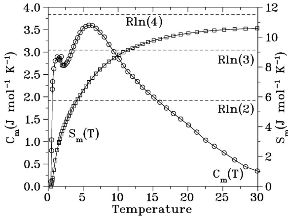
FIG. 7. Magnetic specific heat C_m(T) of \text{Tb}_2\text{Ti}_2\text{O}_7 in zero applied field (circles), and entropy S_m(T) (squares) are shown. The entropy values for two, three, and four states are indicated by the horizontal dashed lines. R is the molar gas constant R = N_0 k_B = 8.3145 \text{ J mol}^{-1} \text{ K}^{-1} . The solid lines are guide to the eye.
