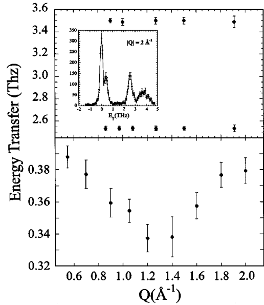
FIG. 4. Inelastic neutron-scattering data obtained at a temperature T = 12 K. The inset of the top panel of Fig. 4 shows a transfer energy scan at Q = 2 \text{ \AA}^{-1} . Data showing representative neutron groups as well as the dispersion relation for these excitations at \sim 2.5 and 3.5 THz is shown in the top panel of Fig. 4. The dispersion of the low-lying excitation is shown in the lower panel.
