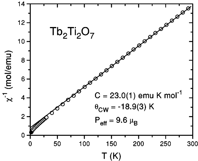
FIG. 2. Inverse molar susceptibility 1/\chi of \text{Tb}_2\text{Ti}_2\text{O}_7 vs temperature.
