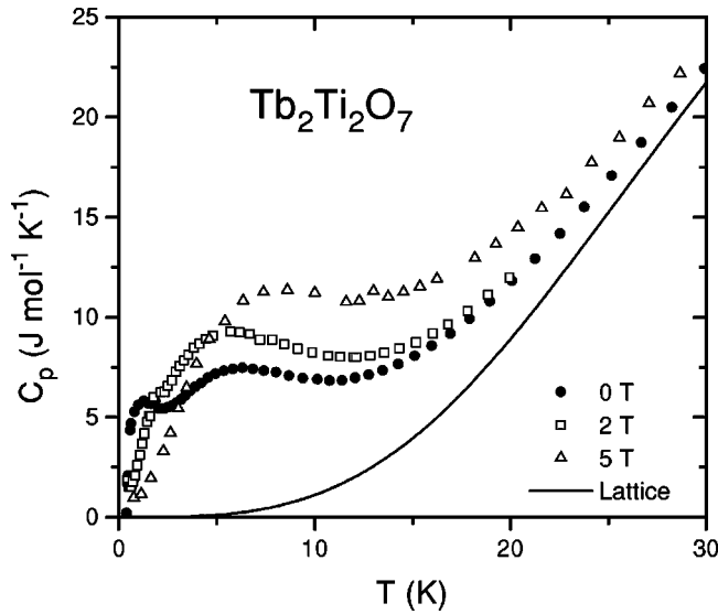
FIG. 5. Specific heat C_p of \text{Tb}_2\text{Ti}_2\text{O}_7 as function of temperature for the indicated magnetic fields of 0, 2, and 5 T. The solid line corresponds to the lattice specific heat of \text{Tb}_2\text{Ti}_2\text{O}_7 , C_l , estimated from the measurements on the nonmagnetic \text{Y}_2\text{Ti}_2\text{O}_7 that is isostructural to \text{Tb}_2\text{Ti}_2\text{O}_7 (Ref. 47).
