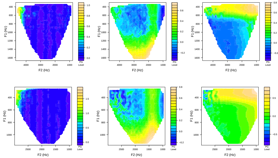
Figure B.6: Vowel category response surfaces Q_5^E(\mathbf{c}, 0.5) (top) and Q_5^E(\mathbf{c}, 10) (bottom) for caretaker E_{10}^5 derived from subject s_5^E ( \mathbf{c} \in \{\mathbf{i}, \mathbf{a}, \mathbf{u}\} ).
