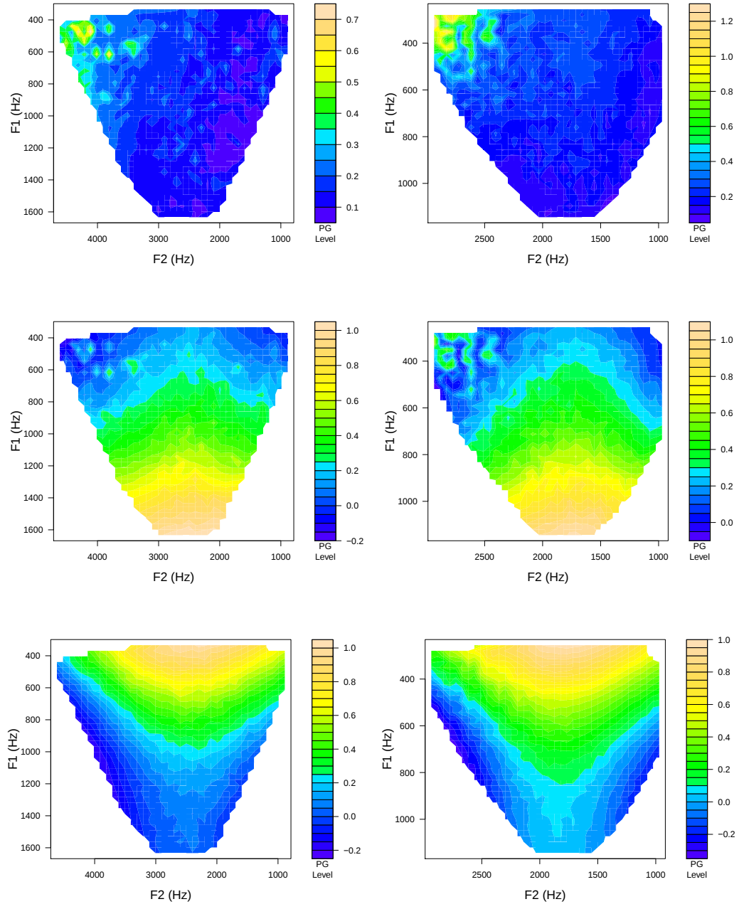
Figure 3.12: Vowel category response surfaces Q_{20}^J(c, 0.5) (left) and Q_{20}^J(c, 10) (right) for caretaker J_{10}^{20} derived from subject s_{20}^J ( c \in \{i, a, u\} ).
