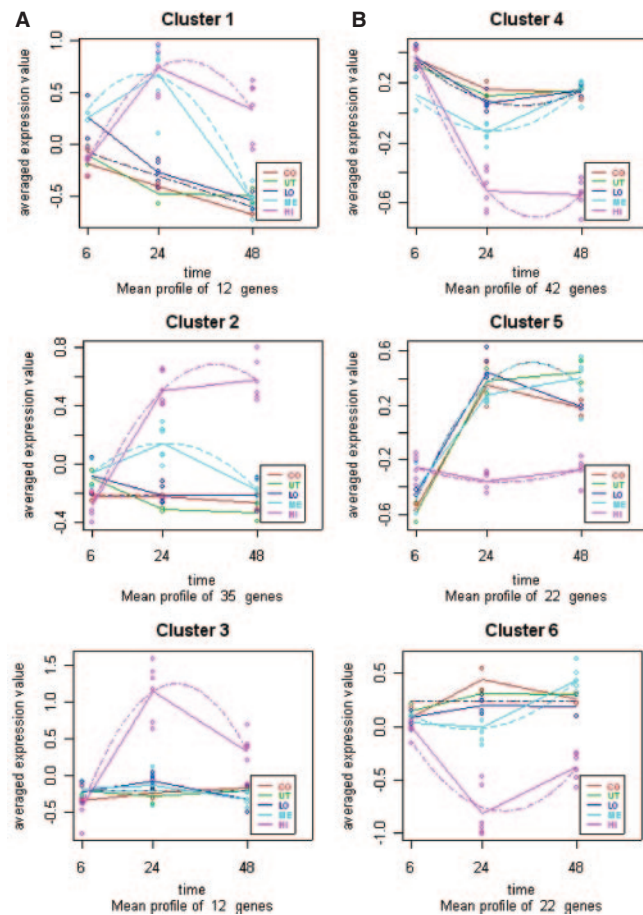
Fig. 2. Data visualization by cluster analysis. Each plot shows the cluster average expression profile by experimental group. (A) Genes with a positive D_{HI} \times T coefficient (induced). (B) Genes with a negative D_{HI} \times T coefficient (repressed). Dots show actual expression values. Solid lines have been drawn joining the average value of gene expression at each time point for each experimental group. Fitted curves are displayed as dotted lines.
