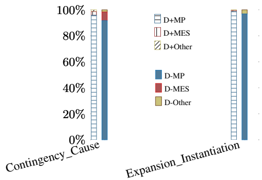
Figure 6: Continuous Case of Implicit Connectives: Graph for Models D+ and D- showing MP (Match Prediction), MES (Mismatch with Explicit Sister type), and Other (Explicit For Implicit Minus One, Minus Two, and Minus Three types)
