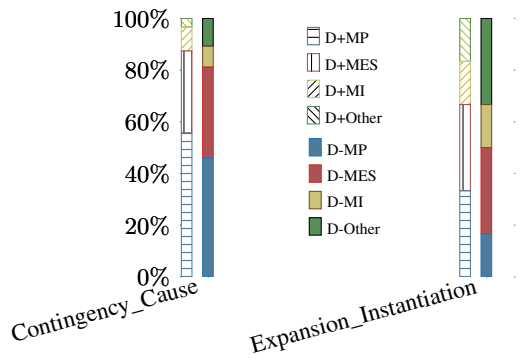
Figure 5: Continuous Explicit Connective Case: Graph for Models D+ and D- showing MP (Match Prediction); MES (Mismatch with Explicit Sister type); MI (Mismatch with Implicit); and Other (Explicit For Explicit Minus One, Minus Two, and Minus Three level types)
