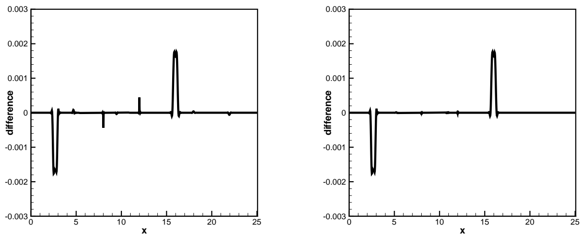
Figure 3.12: Same as in Figure 3.8, but 1000 uniform cells are employed.
