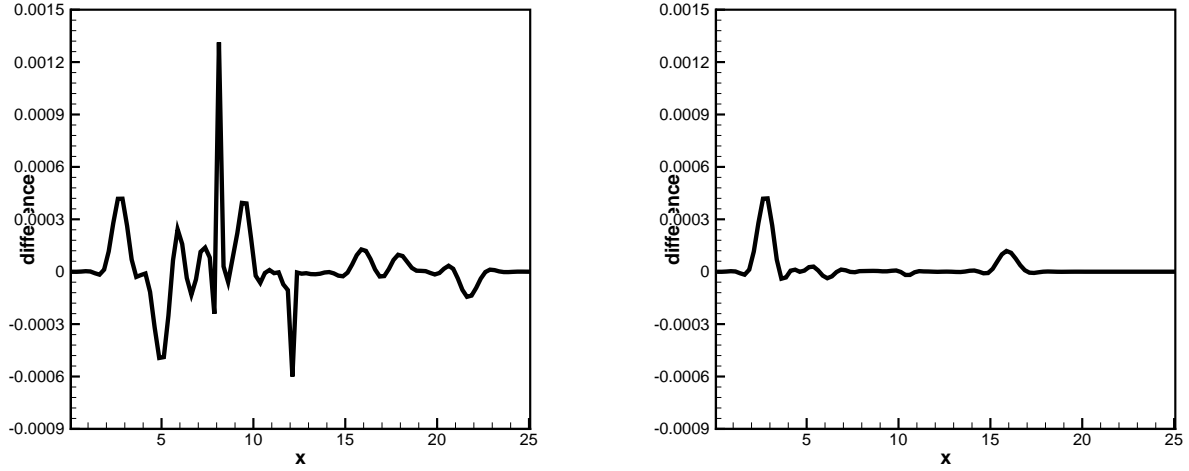
Figure 3.7: The difference between the height h at time t = 1.5 and the background moving steady state water height (3.2), when 100 uniform cells are employed. An initial perturbation of size 0.001 is imposed between [5.75, 6.25] . Left: result based on still-water well-balanced scheme. Right: result based on moving-water well-balanced scheme.
