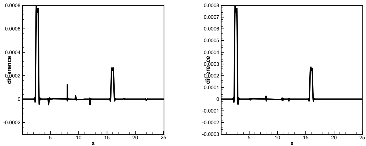
Figure 3.11: Same as in Figure 3.7, but 1000 uniform cells are employed.
