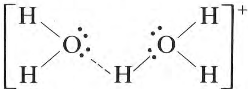
Figure 16.1 The hydrated proton
