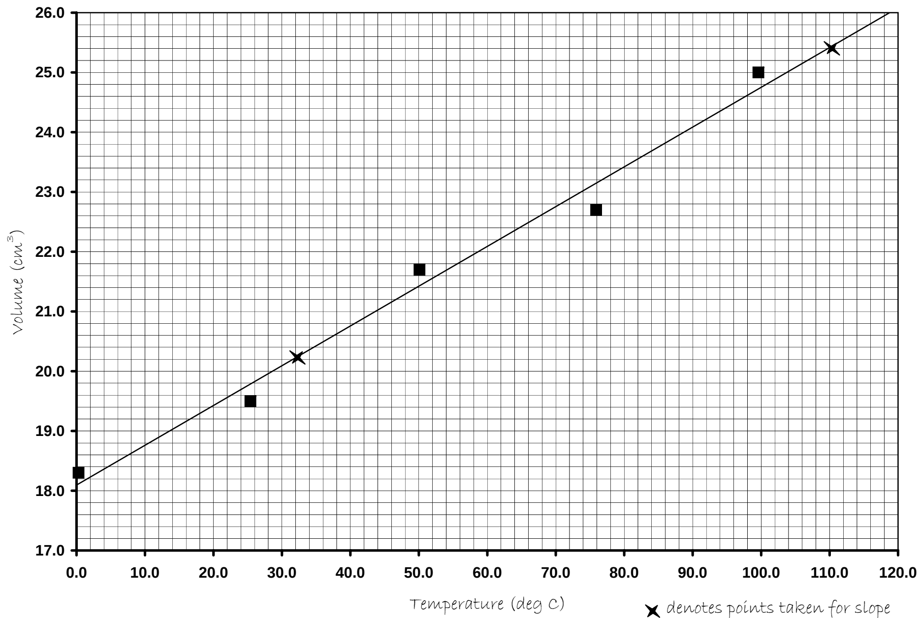
Figure 1: Volume versus Temperature for Part A
